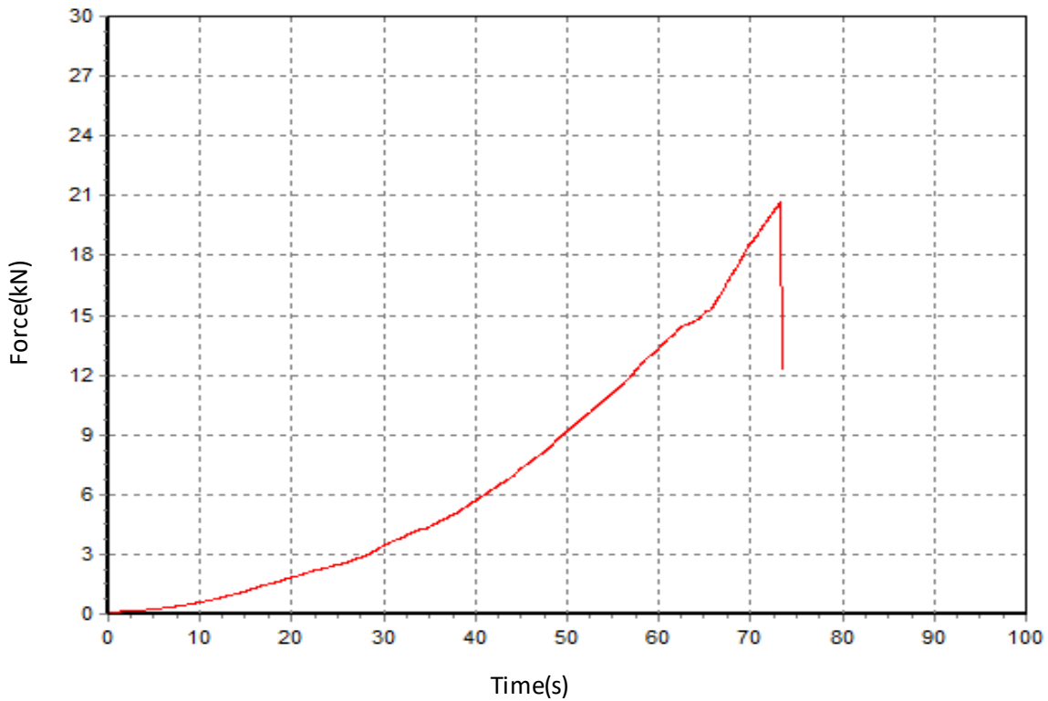
Force-Time Curve
