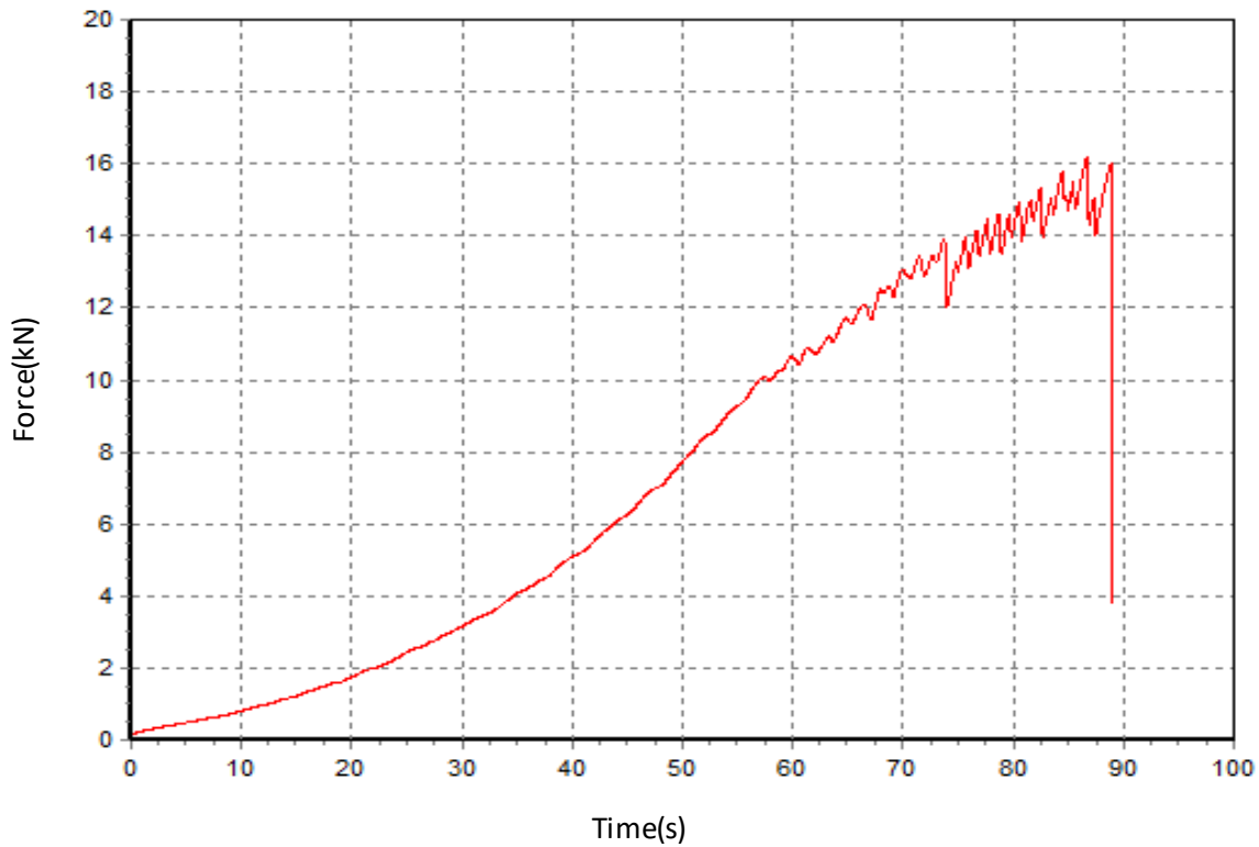
Force-Time Curve
